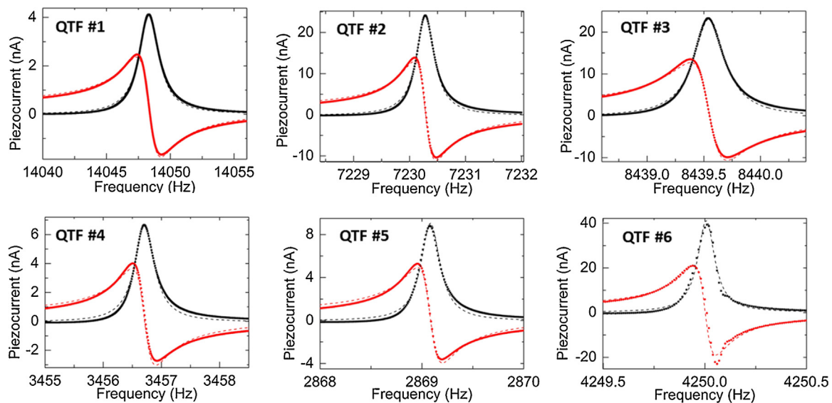
Fig. 4. Resonance curves for in-phase I_a (black dots) and out-of-phase I_b (red dots) components of the QTF current measured at a fixed excitation level V_0 = 0.5 mV and at a pressure of 50 Torr in standard air for custom QTFs near the fundamental oscillation mode. The dashed lines indicate the best-fit curves using Eq. (9). (For interpretation of the references to color in this figure legend, the reader is referred to the web version of this article.)
