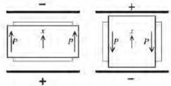
Converse piezoelectric effect
