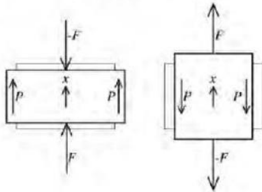
Direct piezoelectric effect
