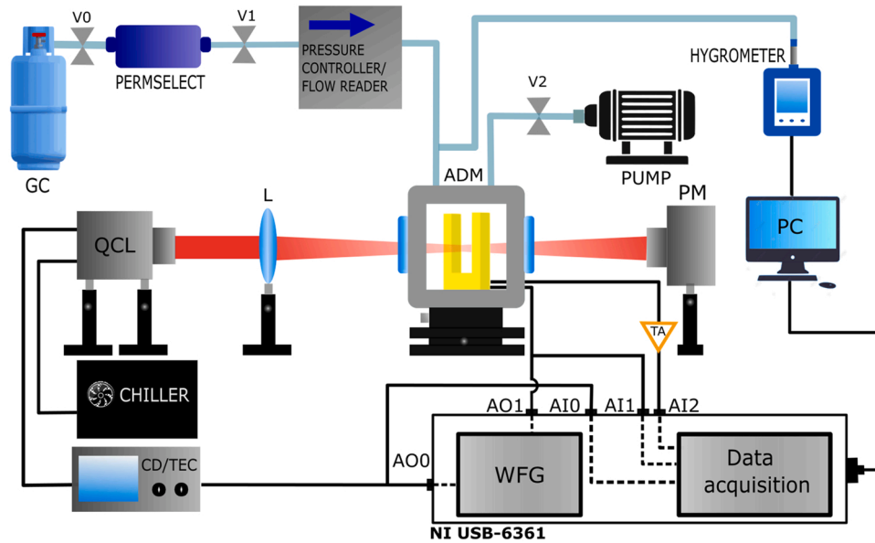
Fig. 1. Schematic of the experimental setup. QCL: quantum cascade laser, TEC: thermoelectric cooler, CD: current driver, WFG: waveform generator, AO0, AO1: analog outputs; AI0, AI1: analog inputs; L: focusing lens, ADM: acoustic detection module, TA: transimpedance amplifier, PM: power meter, V0, V1 and V2: needle valves, DAQ: data acquisition card, PC: personal computer.
