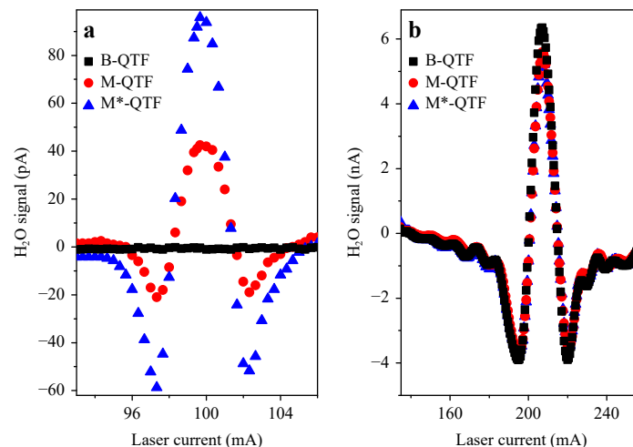
Fig. 4 a 2f spectral-scans of water at 1.39 \mu\text{m} from B (black squares), M (red dots) and M* (blue triangles); b 2f spectral-scans of water at 7.38 \mu\text{m} from B (black squares), M (red dots) and M* (blue triangles).
